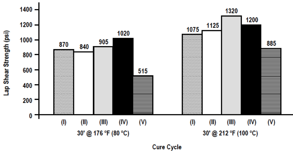
FIGURE 1: LAP SHEAR STRENGTH VS. CURE CYCLE AT 176°F AND 212°F (80°C AND 100°C)
