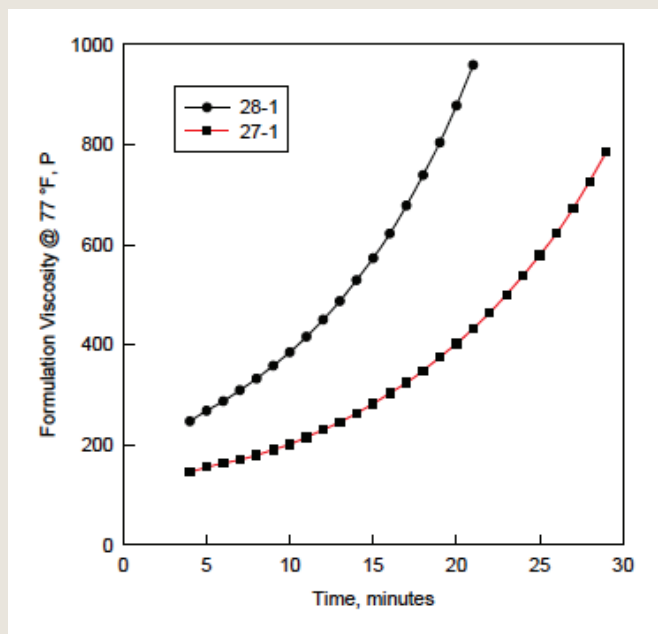
FIGURE 2: VISCOSITY VS. TIME FOR ANCAMINE 2422/EPOXY NOVOLAC FORMULATIONS
