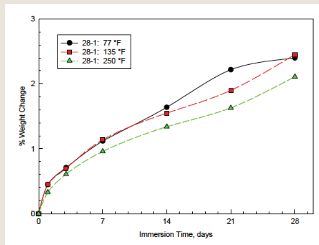
FIGURE 6: 30% NITRIC ACID RESISTANCE OF ANCAMINE 2422/EPOXY NOVOLAC FORMULATION 28-1
