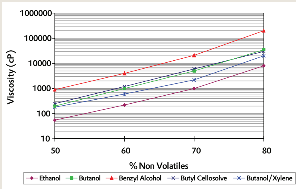
FIGURE 2: VISCOSITY OF ANCAMINE 2410 IN SOLVENTS
