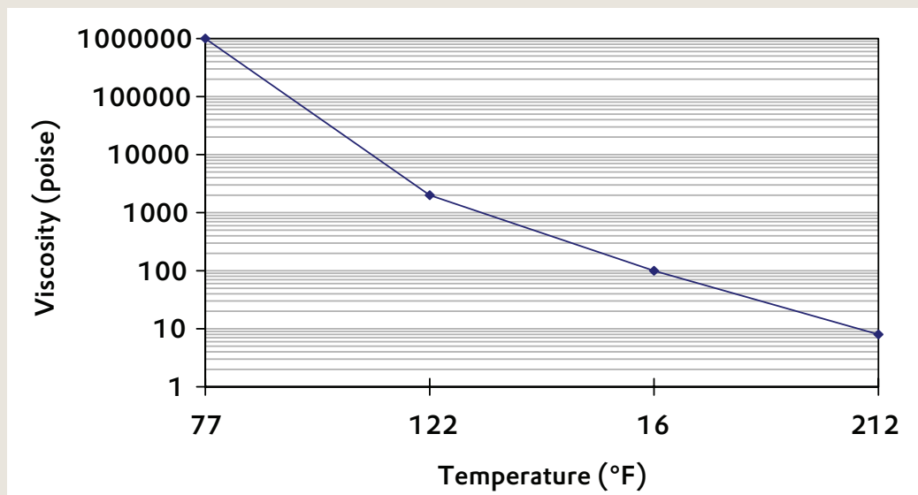
FIGURE 1: ANCAMINE 2410 VISCOSITY
