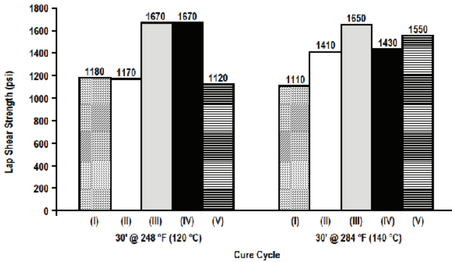
FIGURE 2: LAP SHEAR STRENGTH VS. CURE CYCLE AT 248°F AND 284°F (120°C AND 140°C)
