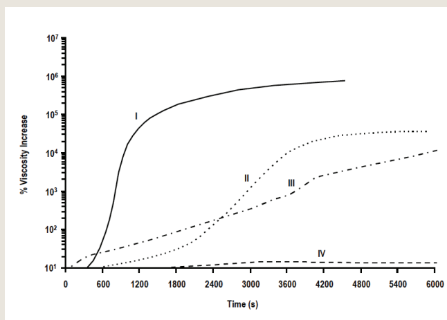
FIGURE 4: VISCOSITY VS. TIME @ 140 °F (60 °C)
