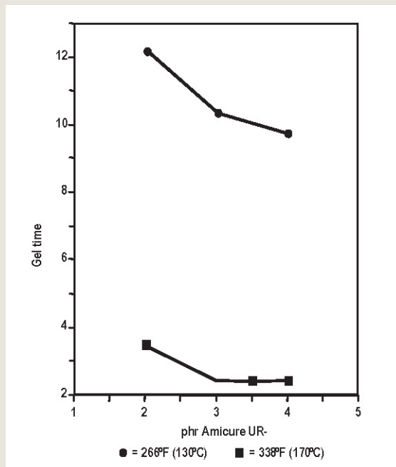
FIGURE 1: GEL TIME VS. PHR OF AMICURE UR7/10
