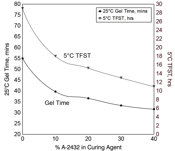
Ancamine 2280-cured LER Accelerated with Ancamine 2432
