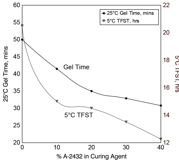
Ancamine 1618-cured LER Accelerated with Ancamine 2432
