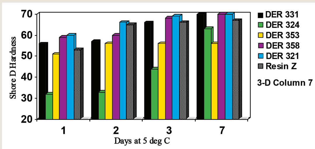
FIGURE 2: EFFECT OF REACTIVE DILUENTS ON ANCAMINE 2432 CURING AGENT REACTIVITY HARDNESS BUILD
