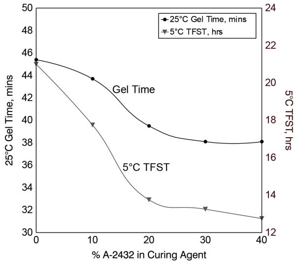
Ancamine 2143-cured LER Accelerated with Ancamine 2432
