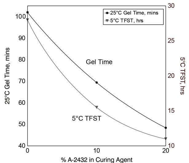
Ancamide 2396-cured LER Accelerated with Ancamine 2432
