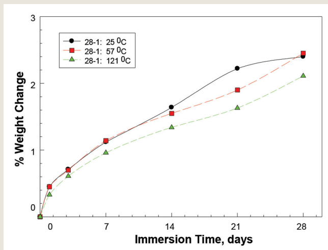
FIGURE 6: NITRIC ACID OF ANCAMINE 2422/EPOXY NOVOLAC FORMULATION 28-1
