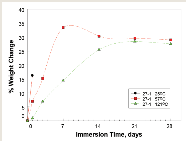
FIGURE 3: METHYLENE CHLORIDE RESISTANCE OF ANCAMINE 2422/EPOXY NOVOLAC FORMULATION 27-1
