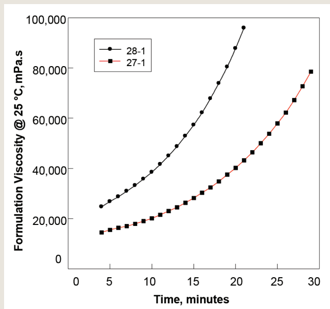
FIGURE 2: VISCOSITY VS. TIME FOR ANCAMINE 2422/ EPOXY NOVOLAC
