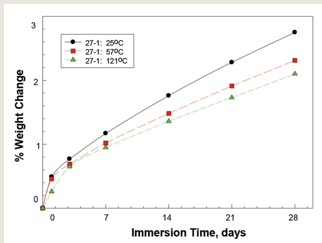
FIGURE 5: NITRIC ACID OF ANCAMINE 2422/EPOXY NOVOLAC FORMULATION 27-1
