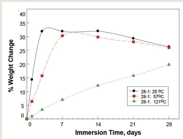
FIGURE 4: METHYLENE CHLORIDE RESISTANCE OF ANCAMINE 2422/EPOXY NOVOLAC FORMULATION 28-1
