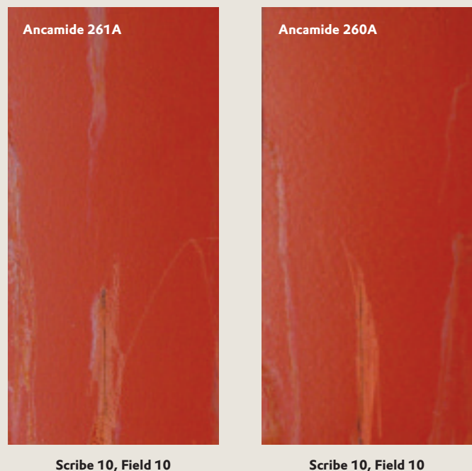
ANCAMIDE 261A AND ANCAMIDE 260A-P1 PRIMERS 1000H SALT SPRAY EXPOSURE
