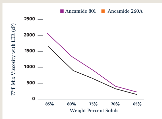
FIGURE 2: VISCOSITY REDUCTION CURVES HIGH EQUIVALENT WEIGHT POLYAMIDES
