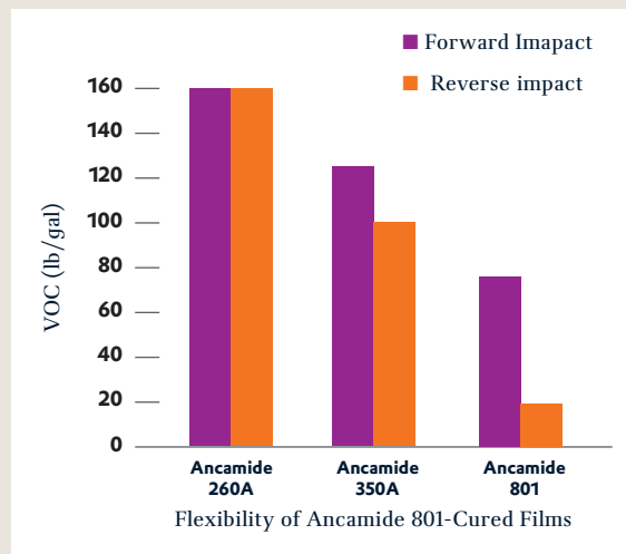
FIGURE 4: IMPACT RESISTANCE OF MODEL CLEARCOATS – 14-DAY CURE
