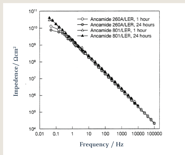
FIGURE 6: EIS FOR ANCAMIDE 801 VERSUS STANDARD POLYAMIDE
