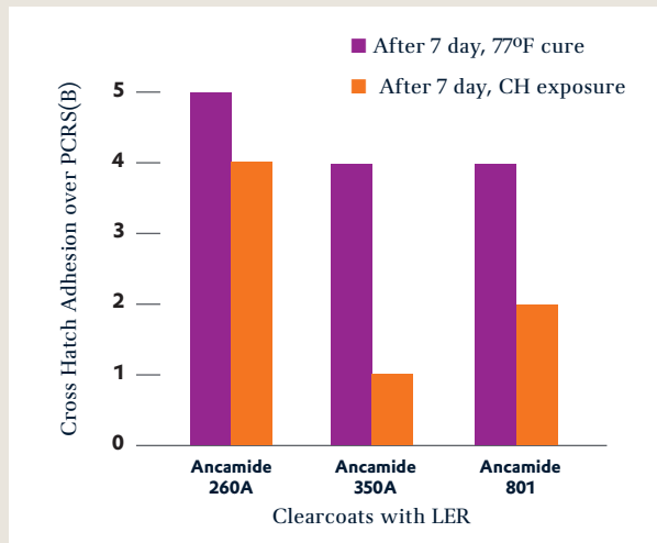
FIGURE 5: CROSS HATCH ADHESION FOR MODEL CLEARCOATS
